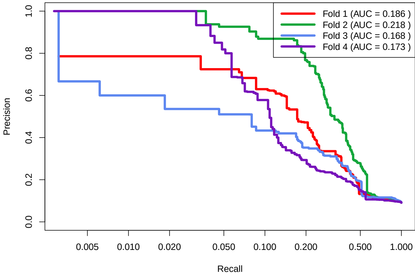
SPELL All Datasets:113x20x1Training
